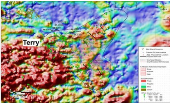
Figure 3: Reduced to pole analytical signal magnetics map, with high potassic signature outline and 2022 proposed drill hole locations (CNW Group/Libero Copper & Gold Corporation.)
