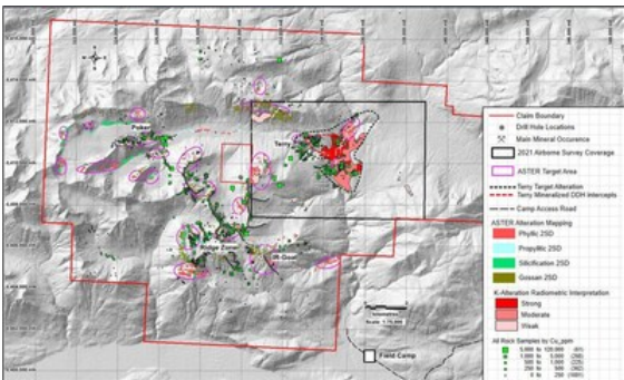
Figure 5: Gray scale DEM backdrop, large K-enrichment area immediately southeast of the Terry porphyry Cu-Au discovery, ASTER target areas and rock sample geochemistry (Cu ppm) (CNW Group/Libero Copper & Gold Corporation.)
