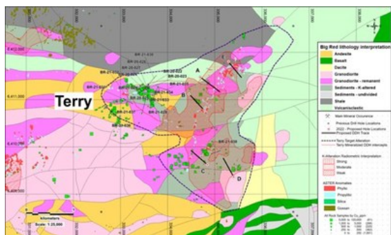
Figure 1: Geological interpretation map (from 2021 airborne data), strong potassic alteration located immediately southeast of the Terry porphyry Cu-Au discovery, with 2022 proposed drill hole locations (CNW Group/Libero Copper & Gold Corporation.)
