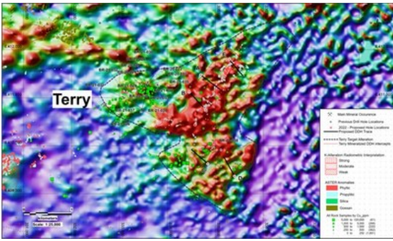
Figure 2: K/Th ratio map (2021 radiometric survey data), strong potassic alteration immediately southeast of the Terry porphyry Cu-Au discovery. with 2022 proposed drill hole locations (CNW Group/Libero Copper & Gold Corporation.)
