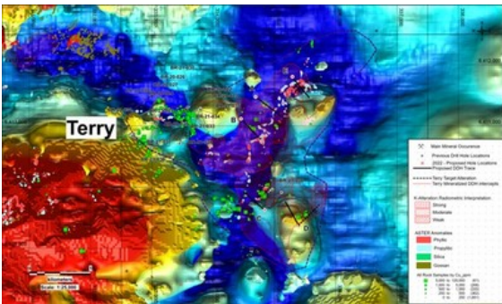
Figure 4: Magnetic inversion model isosurface map with smaller apophyses flanking both the area with potassic enrichment and large magnetic low (possible hydrothermal source for the Terry area mineralization) with 2022 proposed drill hole locations (CNW Group/Libero Copper & Gold Corporation.)
